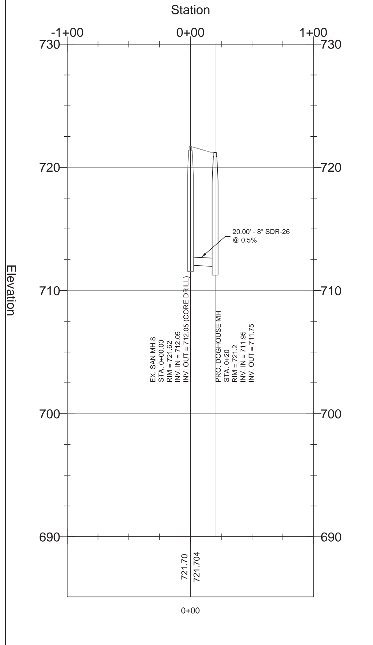
EX. MH 8 TO PROP. MH PROFILE
