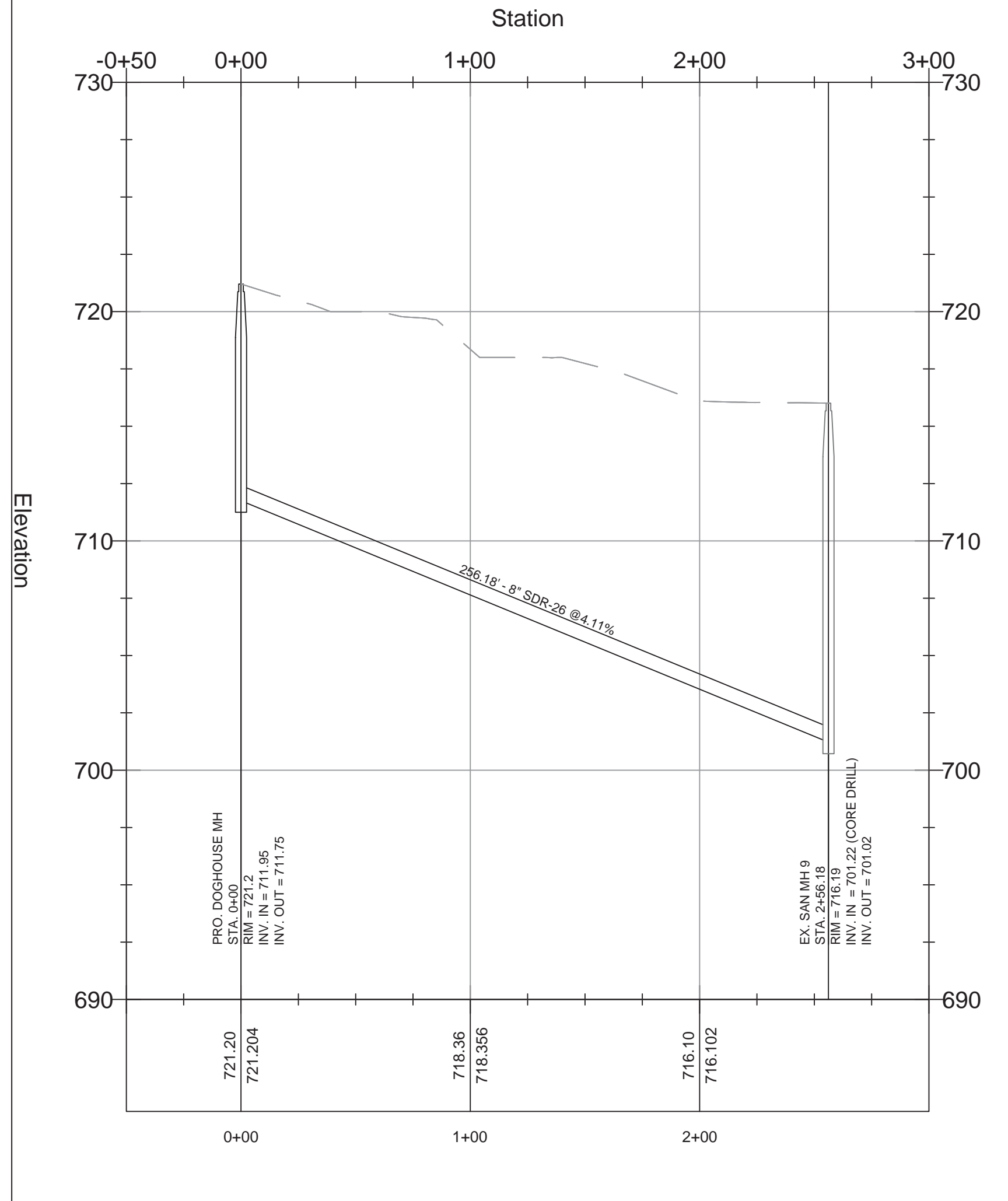
PROP. MH TO EX. MH 9 PROFILE
